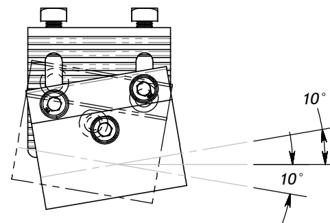
ANGLED POSITION
