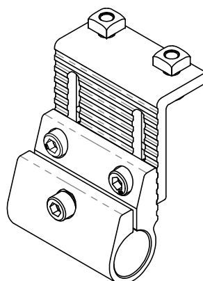
LOW POSITION
