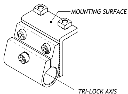
HIGH POSITION
